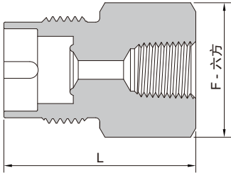
NPT 阴螺纹
